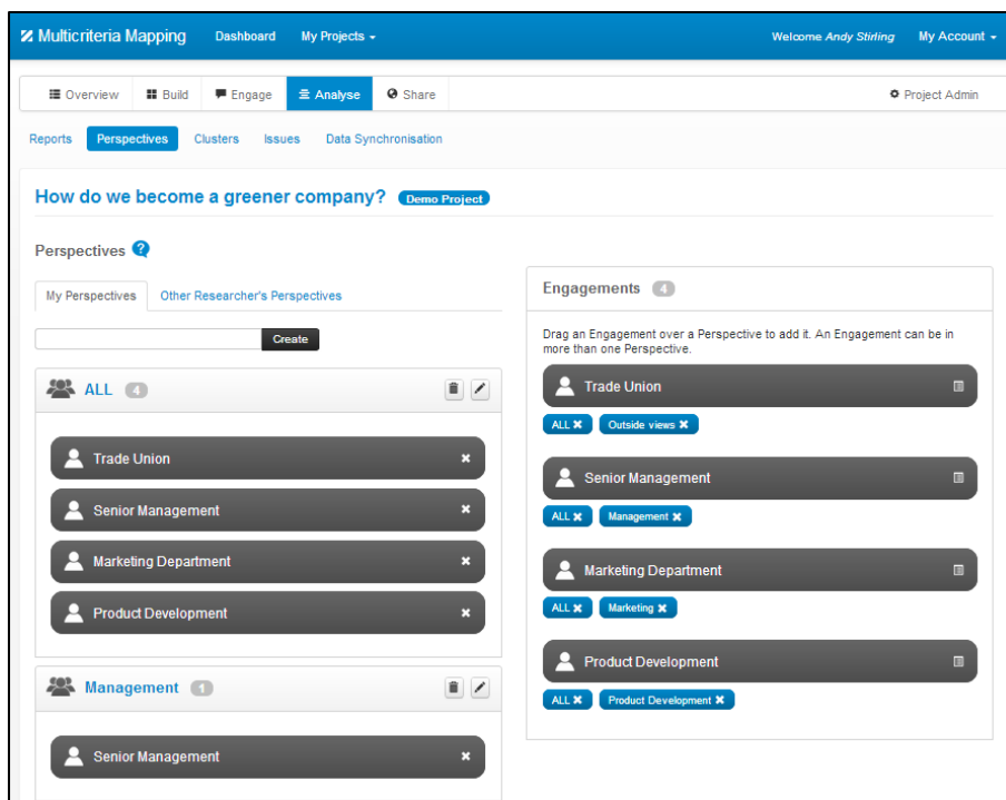
Figure 21: Creating perspectives
