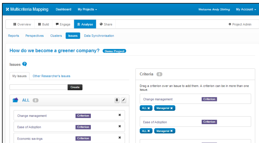
Figure 22: Creating Issues
