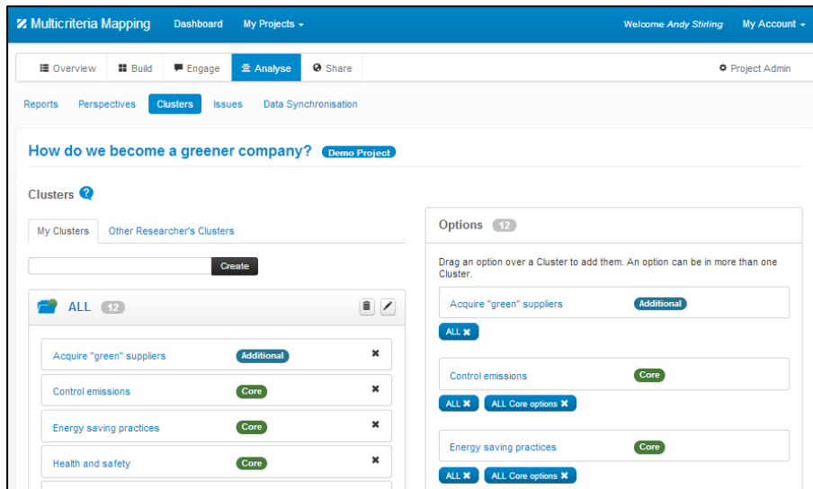
Figure 23: Creating clusters
